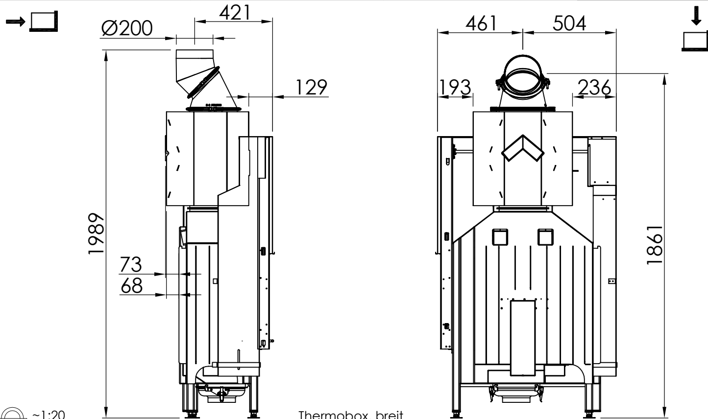
Thermobox, schmal
